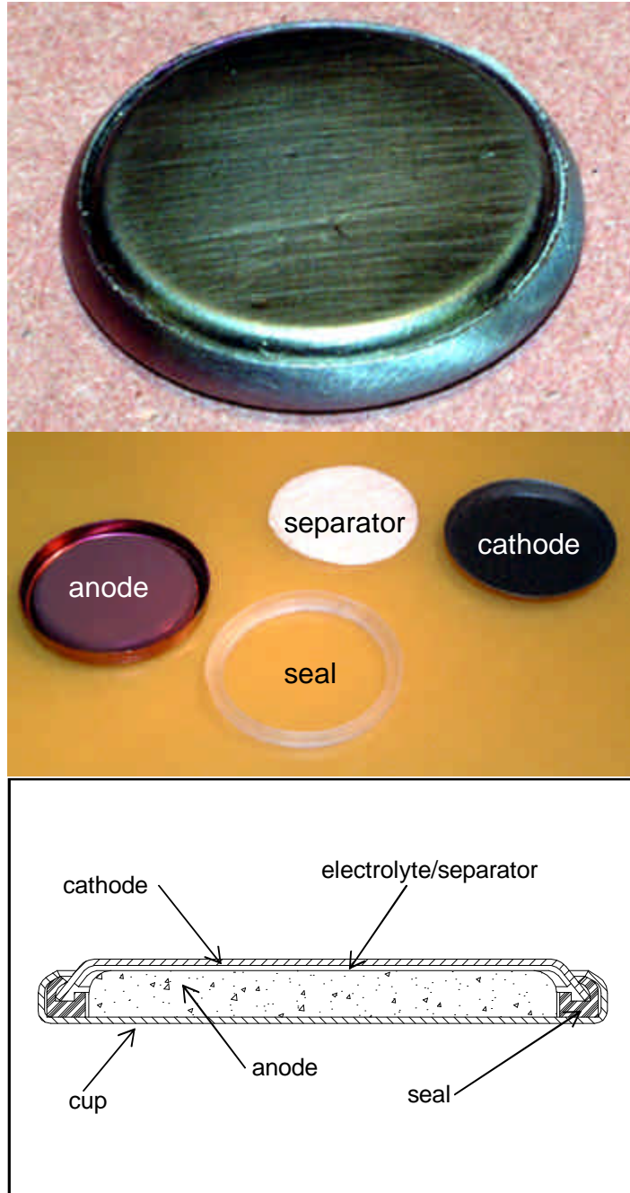
Figure 3. Cross section view of button cell showing major components. The case top and bottom are made from tantalum. The capacitor is assembled dry, and electrolyte is admitted by vacuum impregnation process. Final seal is secured by crimping the exterior perimeter of the anode cup.
