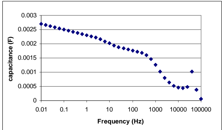
Figure 4. Capacitance vs. frequency for 50 volt button cell. The capacitance is 1750uF at 120Hz.
