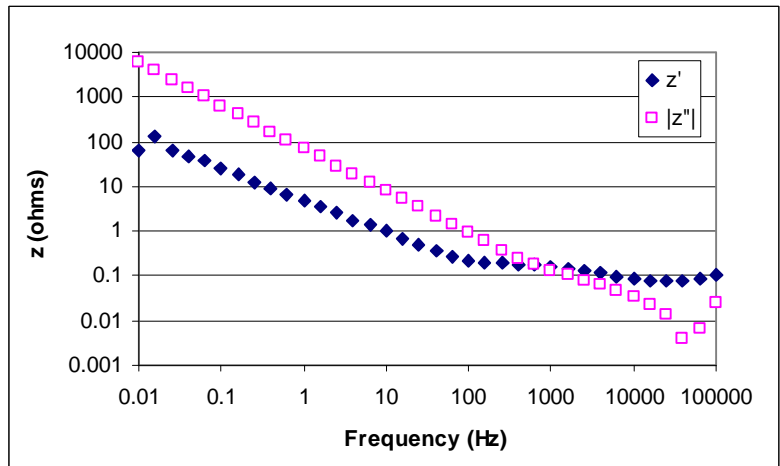
Figure 5. Impedance vs. frequency for 50 volt button cell. The ESR is 161mohm at 1kHz.
