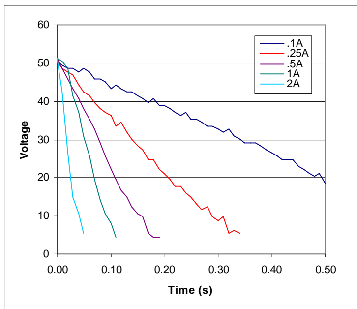
Figure 8. Plot of voltage vs. time for various constant current discharges of the 50V button cell. Capacitance equals the slope of the curve divided
