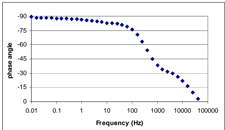
Figure 6. Phase angle vs. frequency for 50 volt button cell. The capacitor has a phase angle of -45^\circ at a frequency of 630Hz. At lower frequencies, the phase angle rapidly approaches -90^\circ .
