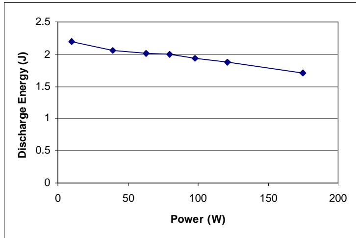
Figure 7. Ragone plot for the 50V 2325 button cell prototype. The maximum load power of 175W represents the limit of the electronic load used to make the measurements. The peak power capability of the capacitor is much higher.
